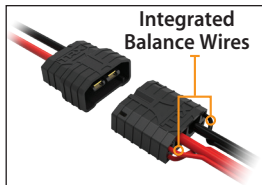
Traxxas High-Current Connector with iD and integrated balance wires (4S shown)
